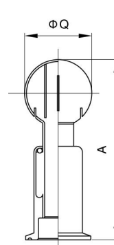
Threaded Rotary Cleaning Ball 3162004
