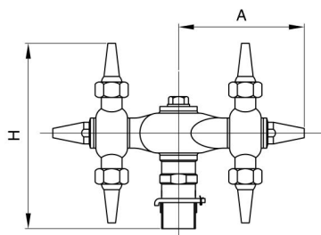
Bolted Rotary Cleaning Ball 3160010
