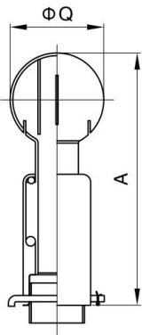
Bolted Rotary Cleaning Ball 3160002
