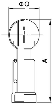
Threaded Rotary Cleaning Ball 3163001
